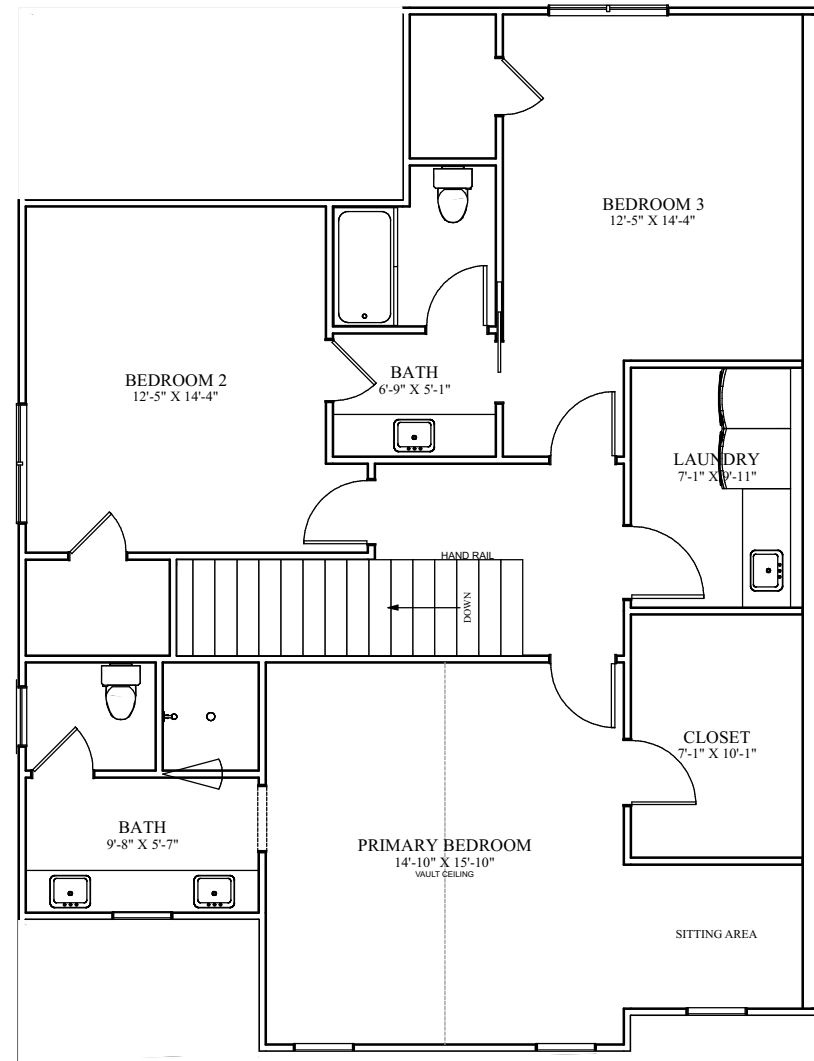
3 A-1 2nd LEVEL PLAN 1/8" = 1'
