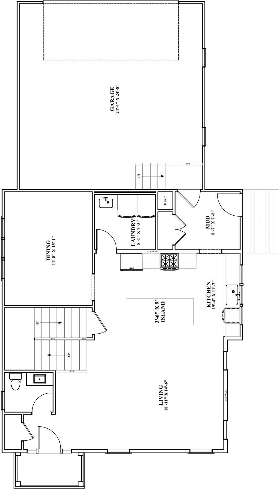
2 A-1 MAIN LEVEL FLOOR PLAN 1/8" = 1'
