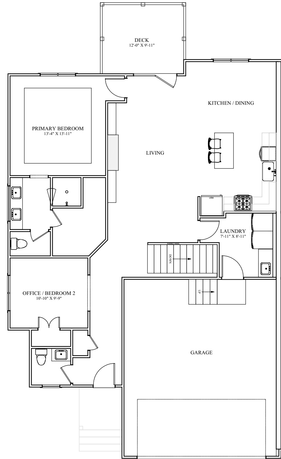
1 A-1 MAIN LEVEL FLOOR PLAN 1/8" = 1'
